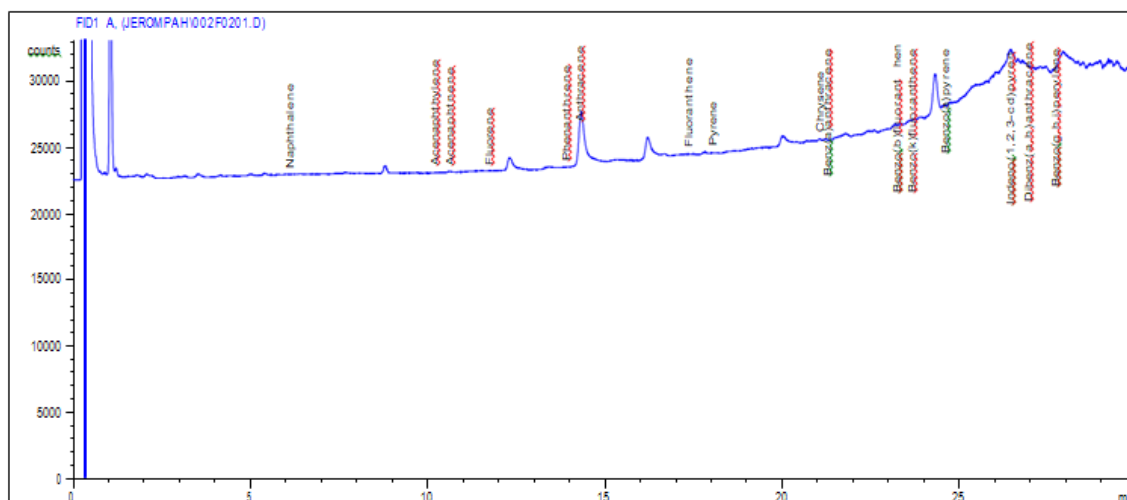
Fig. 6. Chromatogram for the Polyaromatic Hydrocarbons from the Gills of the tilapia specie
